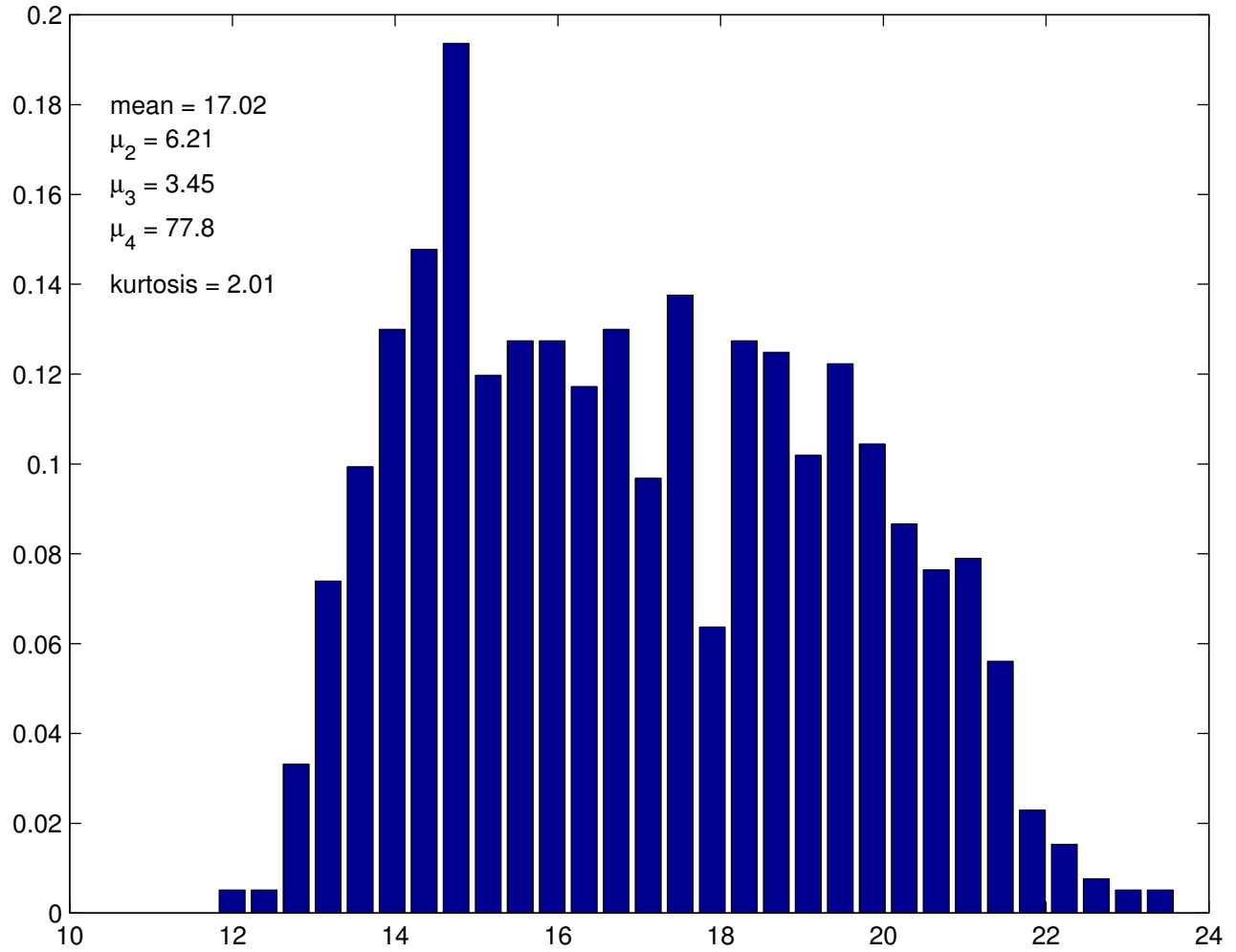
PDF of SST, 1916–1999, monthly means
