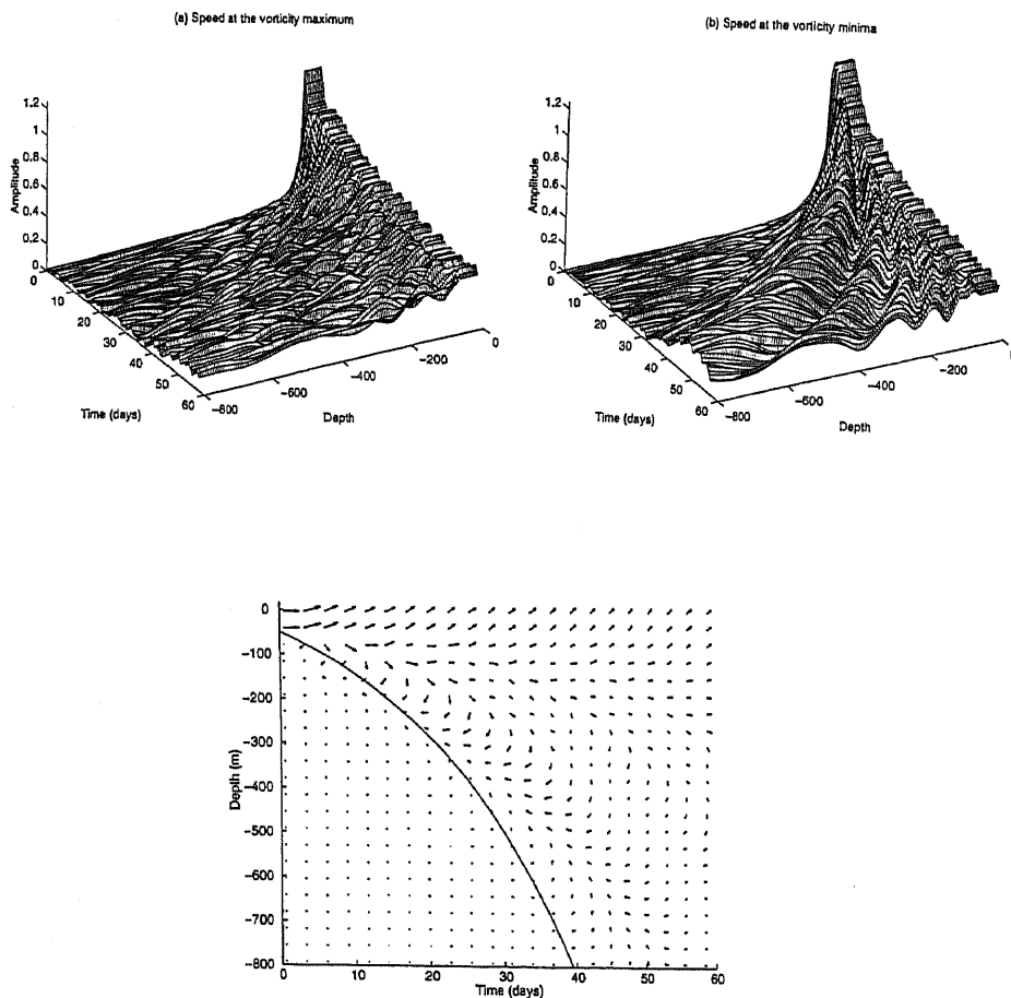
Figure 15. An illustration of the radiation of a near-inertial wave train from the mixed layer. (a) Speed as a function of depth (meters) and time (days) below the vorticity maxima, \eta = 0 and \pi . (b) Speed as a function of depth and time below the vorticity minima, \eta = \pi/2 . The wave train is apparent only below the vorticity minimum. (c) Another view of the near-inertial activity below the vorticity minimum; the arrows indicate the backrotated velocity, L\mathcal{A} = \exp(i\gamma_0 t)(u + iv) , superposed on a depth-time plot. The solid curve is the trajectory in (5.12). Notice the reversal in direction with depth of the near-inertial velocity.
