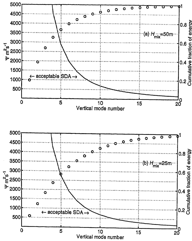
Figure 17. The figure above can be used to estimate the fraction of the energy which is contained in modes which are acceptably described by the strong dispersion approximations. The solid curve is q = 2 (that is, \Psi = f_0^2 h_n^2 ) as a function of the vertical mode number, n . This curve depends on the parameters used to specify the model buoyancy profile in (4.1); shown above are two examples with different values of H_{mix} as indicated. (The other parameters are given in Table 1.) The circles and right-hand ordinate show the cumulative fraction of energy contained in modes with vertical mode number less than or equal to n .
