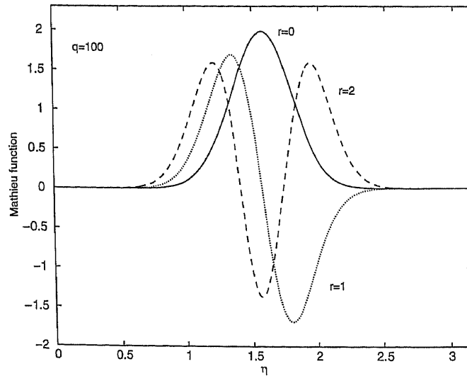
Figure 2. The three Mathieu functions ce_0(\eta, 100) , ce_1(\eta, 100) and ce_2(\eta, 100) . As the index, r , increases the function becomes less localized. Notice also that ce_1 is antisymmetric around \eta = \pi/2 . This antisymmetry ensures that ce_1 does not project onto 1 in the sum (3.11a).
