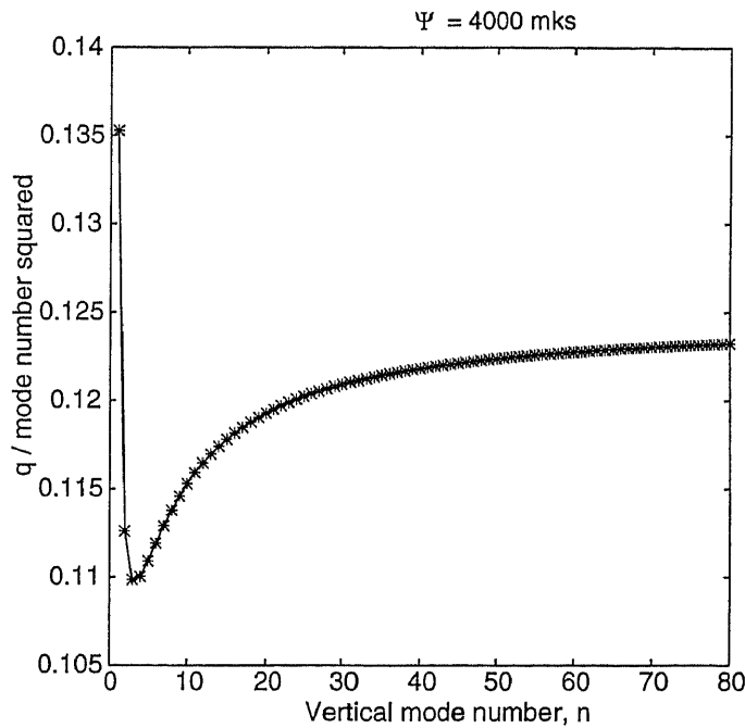
Figure 5. A plot of 2\Psi/n^2 R_n^2 f_0 versus vertical mode number n . The modal speed c_n = f_0 R_n is the eigenvalue obtained from solving the vertical eigenproblem in (4.1) and (4.2). We use the numerical values from Table 1; i.e., \Psi = 4000 \text{ m}^2 \text{ s}^{-1} . Using the combination q/n^2 on the vertical axis removes the strongest dependence on the vertical mode number.
