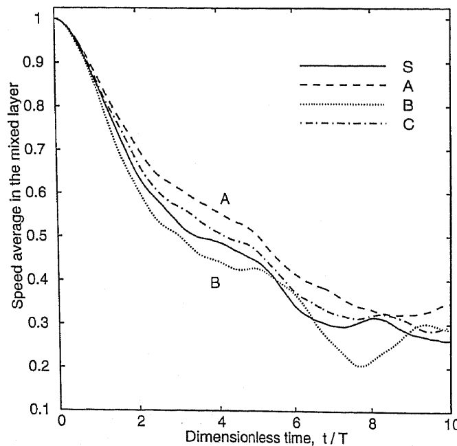
Figure 13. Evolution of the speed, \sqrt{\langle u \rangle^2 + \langle v \rangle^2} , for the four parameter sets (A, B, C and S) in Table 2. Y = 3.302 in all cases, while \mu and \hat{H} have large variations.
