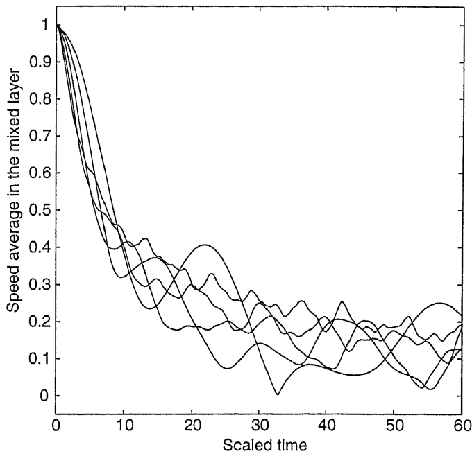
Figure 19. Speed averaged in the mixed layer against the scaled time t/T_1 where T_1 is defined in (6.14) for five calculations with Y = 1.651, 3.302, 6.604, 13.21 and 26.42 . H_{\text{mix}} and N_{\text{mix}} are as in the standard case.
