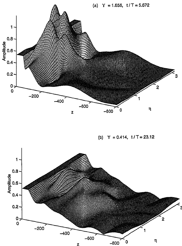
Figure 14. Snapshots of the speed, |L \cdot \nabla(y, z, t)| = \sqrt{u^2 + v^2} , as a surface plot above the (\eta, z) plane. The two calculations above, and the one in Figure 9c, all have \sqrt{\langle u \rangle^2 + \langle v \rangle^2} = 0.54 in the mixed layer. The value of Y and the nondimensional time is indicated on the figure. As Y is increased, the horizontal structure of the fields becomes more complex. When Y is small, as in Figure 14b, the relatively weak horizontal modulations indicate that the strong dispersion approximation of Section 6 is valid.
