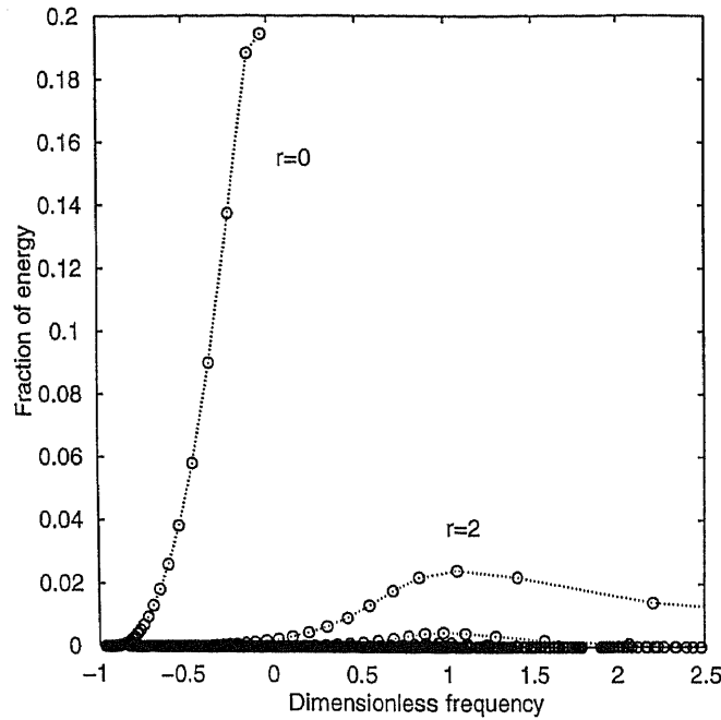
Figure 8. The fraction of energy in mode (2r', n) , \mathcal{E}_{2r',n} in (4.11), plotted against the nondimensional modal frequency, 2\omega_{2r',n}/\zeta_{\min} . The horizontal axis is truncated at \hat{\omega} = 2.5 ; there are higher frequencies in the series (4.8).
