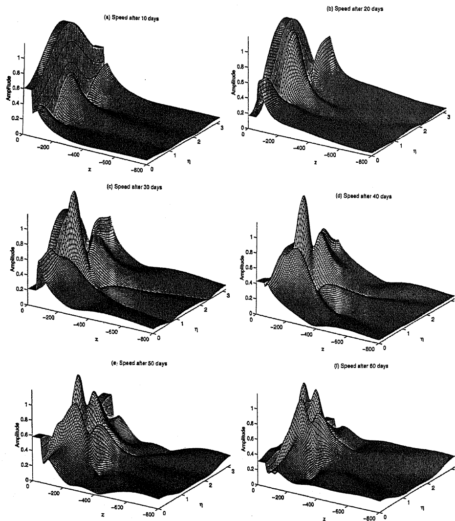
Figure 9. Panels (a)–(f) show snapshots of the speed, |L\mathcal{A}(y, z, t)| = \sqrt{u^2 + v^2} , as surface plots above the (\eta, z) plane every 10 days after the initiation of the near-inertial oscillation. The depth z is in meters and \eta = 2\alpha y is dimensionless.
