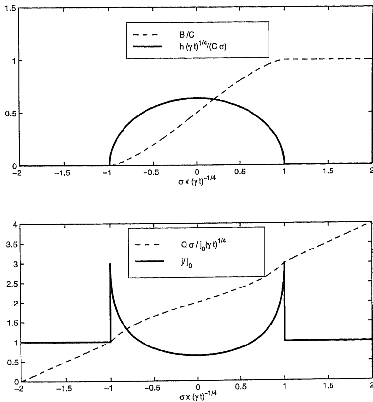
Figure 3. Self-similar solutions of the Eqs. (4.3). (Upper panel) Scaled profiles of buoyancy B and buoyancy gradient h . (Lower panel) Scaled profiles of spice Q and spice gradient j .
