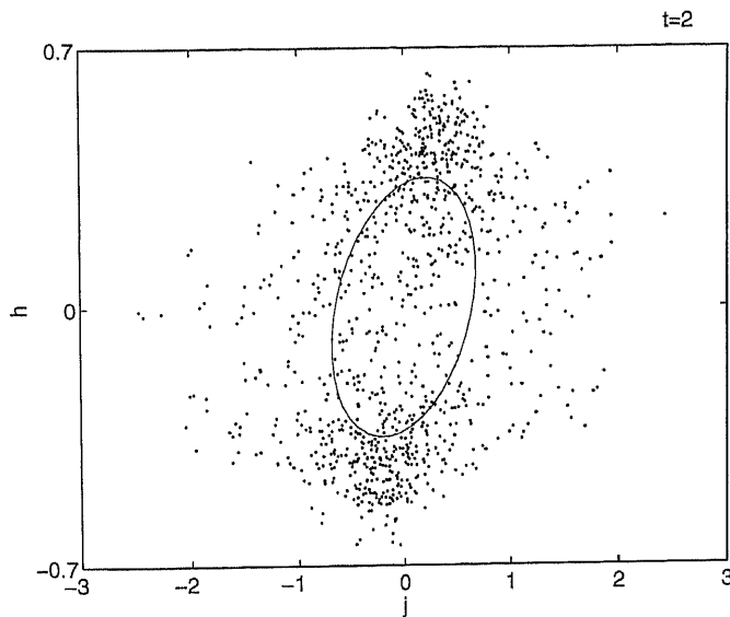
Figure 11. A detailed view of the S_x - T_x diagram of Figure 10d. The axis have been rotated and scaled anisotropically. The best-fit ellipse is tilted with respect to the compensation line (which is the horizontal axis in this figure). The anisotropic scaling of the coordinates reveals the compensation between typical points in the middle of the cloud.
