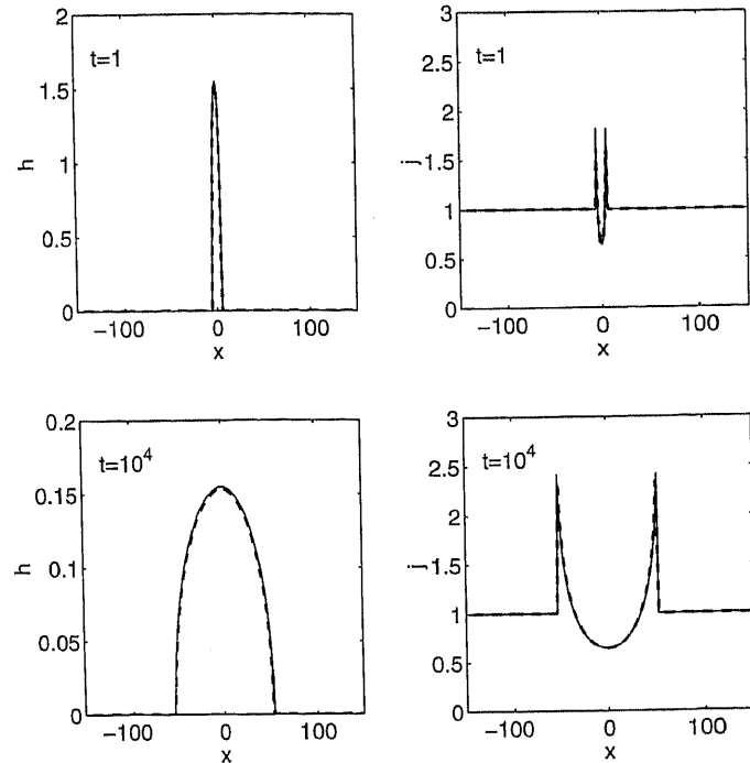
Figure 4. Comparison of numerical (dashed line) and analytic (continuous line) solutions of the coupled thermohaline equations (4.3). The initial conditions for h are given by (4.4) evaluated at t = 10^{-2} with C = 13.06 . The initial condition for j is simply j = 1 everywhere. The peak of h falls exactly on a grid point. The grid spacing is equal to 1. (Left panels) Comparison of the numerical results and the analytic solution (4.4) at t = 1 and t = 10^4 . (Right panels) Comparison of the numerical results and the analytic solution (4.5) at t = 1 and t = 10^4 . The discrete space grid does not completely resolve the two j -spikes (whose maximum value is 3).
