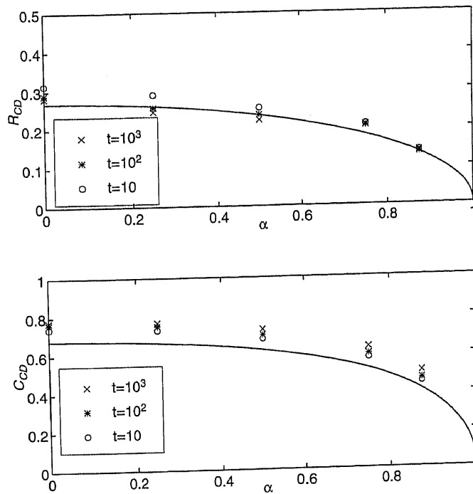
Figure 17. A comparison between the analytic expressions in (4.26) (the continuous curves) and the results of numerical simulation at three different times. All of the simulations have 10,000 points. The agreement between simulation and analysis is consistently better in the upper panel than in the lower panel. In the lower panel, as time increases, the results of the simulation move systematically away from the analytic expression. Notice also the different vertical axis scales between the upper and lower panels.
