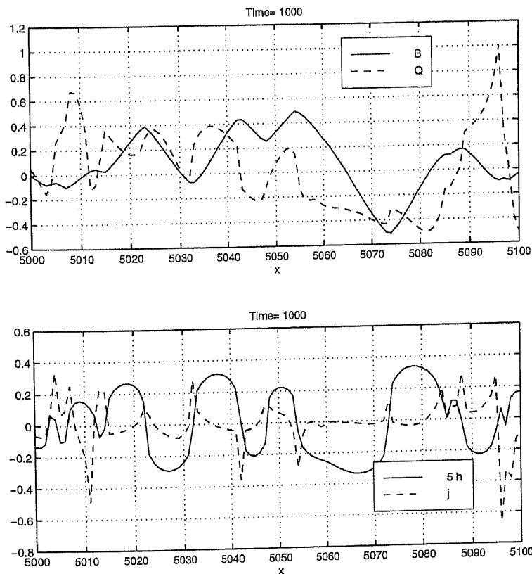
Figure 7. Profiles of B and Q (upper panel) and h and j (lower panel) at t = 1000 for the same simulation and subsection shown in Figure 6.
