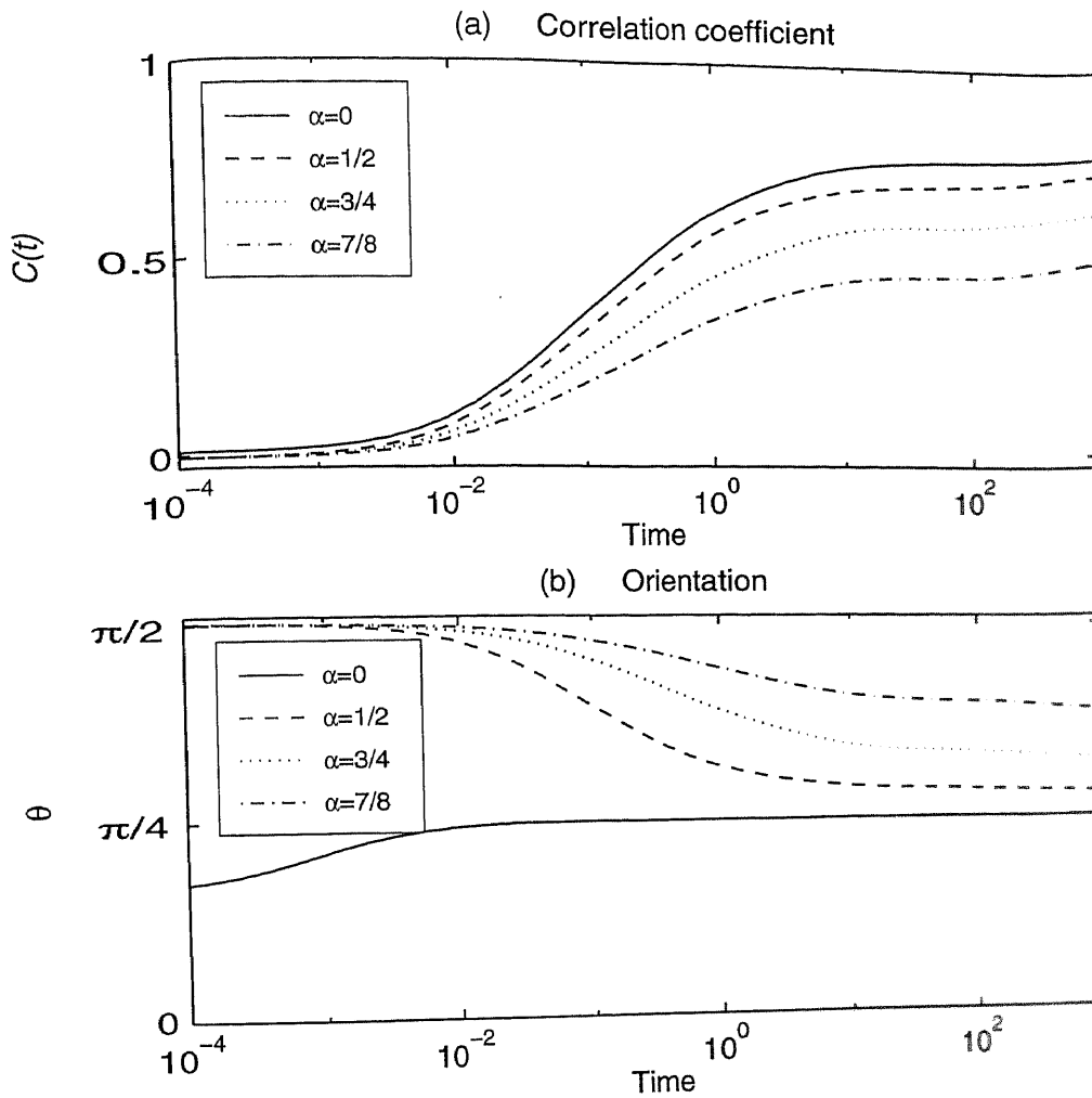
Figure 13. (a) Evolution of the correlation coefficient C(t) defined in (4.17b) (b) Evolution of the orientation of the best-fit ellipse in the T_x - S_x plane. The initial condition is the same as that of Figure 12.
