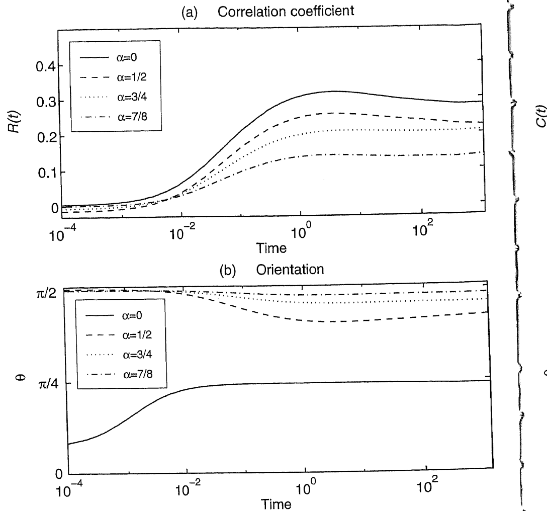
Figure 12. (a) Evolution of the correlation coefficient R(t) defined in (4.17a). (b) Evolution of the orientation of the best-fit ellipse in the (S, T) plane. The initial conditions is 10,000 (S, T) points selected from uniform probability densities with variances (1 + \alpha)/2 and (1 - \alpha)/2 respectively. For \alpha = 0 the orientation is always close to \pi/4 except for an initial transient due to random asymmetries in the initial conditions. For \alpha \neq 0 , \theta(0) = \pi/2 ; then as the time increases, \theta(t) decreases and approaches a steady value which is a function of \alpha . If \alpha \neq 0 , the orientation is steeper for the fields than for the gradients.
