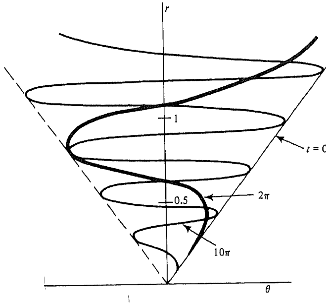
FIGURE 2. The dependence of the advected tracer concentration \theta_A (at \phi = 0 ) on radius for the angular velocity field \Omega(r) = \exp(-r^2) , with \theta(t=0) = r \cos \phi . The wavelength of the concentration decreases like t^{-1}\Omega_r .
