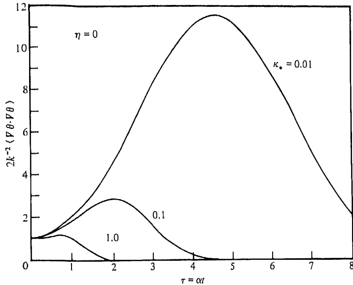
FIGURE 1. The mean-square tracer gradient as a function of time, for various \kappa_* \equiv \kappa k^2 / \alpha . The ordinate is proportional to the dissipation rate for variance of \theta .
