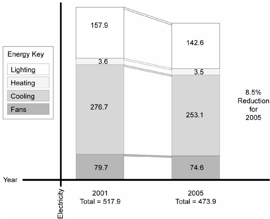
Figure 1-2 – Demand Savings Related to the 2005 Standards
