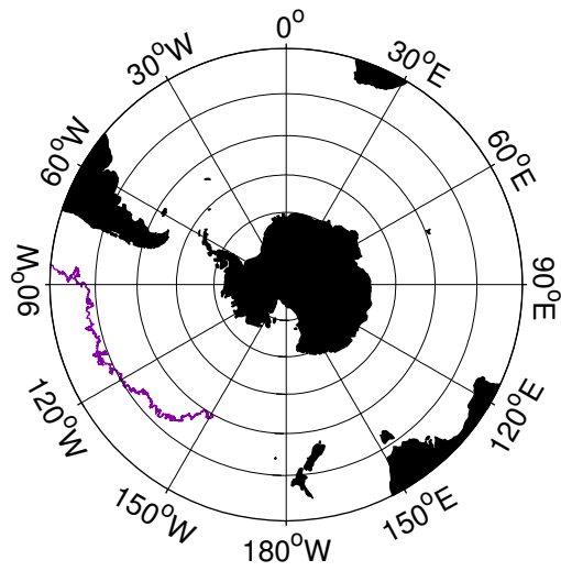
drifter trajectory from June 1 1996 to June 27 2000
