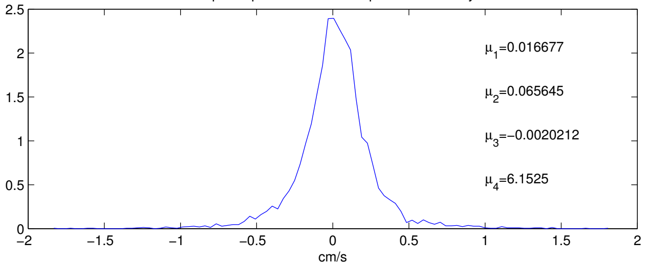
empirical pdf for drifter v component of velocity
