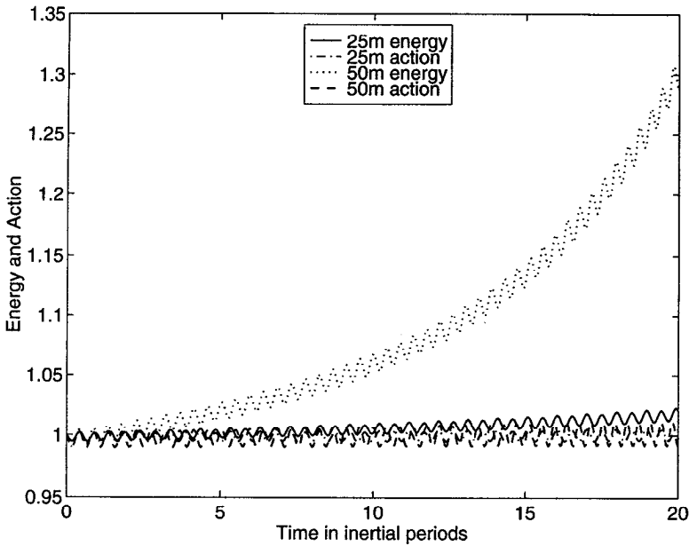
Figure 1. Energy and action obtained by numerically integrating (4.14) with k = l = 2\pi/20 km, f_0 = 10^{-4} s ^{-1} , s = 2f_0 and N = 100f_0 . With both m_0 = 2\pi/50 m and m_0 = 2\pi/25 m the action is more nearly constant than the energy.
